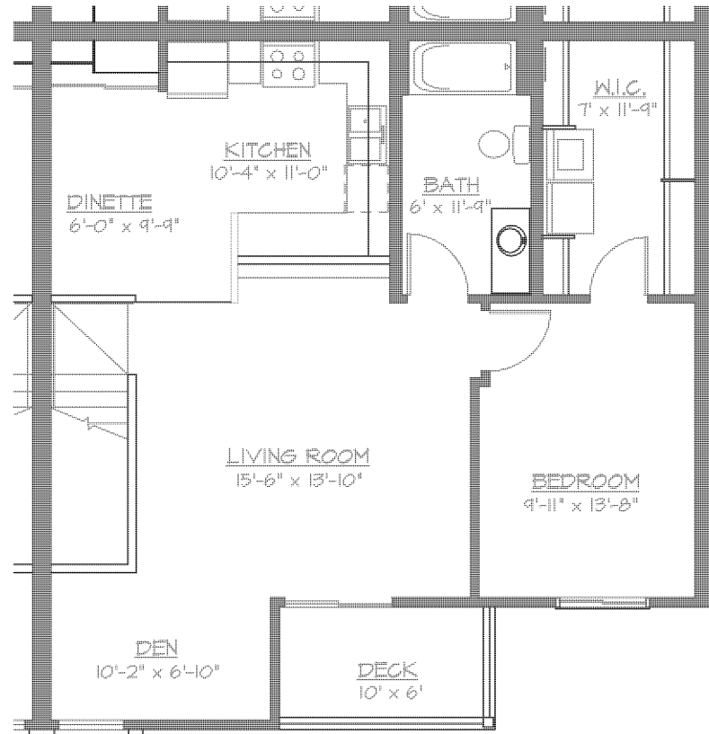
Detailed Floor Plan - 7320, 7380, 7410 UNITS #3, 6, 11, 14
