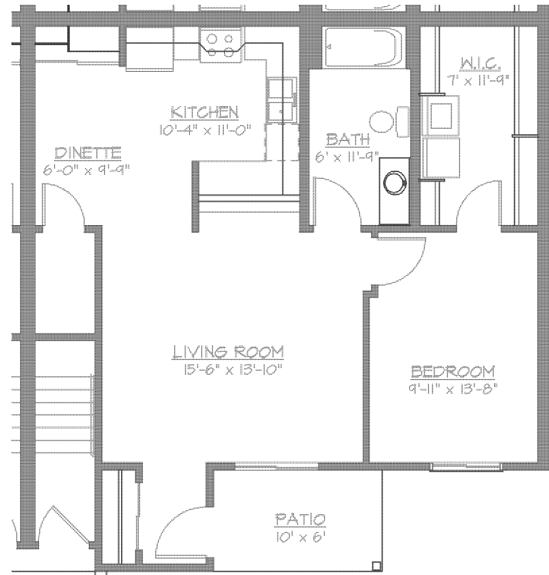
Detailed Floor Plan - 7320, 7380, 7410 UNITS #4, 5, 12, 13
